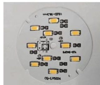
High Bright 5730 Chips Total 10x0.5W=5W
